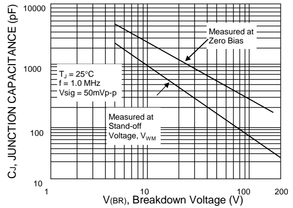
FIG. 2 - TYPICAL JUNCTION CAPACITANCE UNI-DIRECTIONAL
